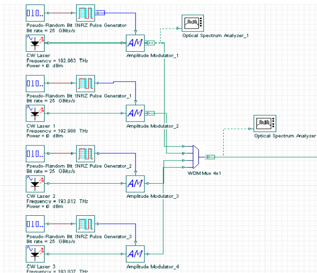
Fig. 7. 4x25 Gbps optical communication system.
