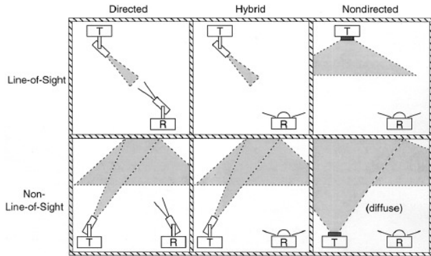
Fig. 1 Classification of simple infrared LOS and non-LOS links [1].
