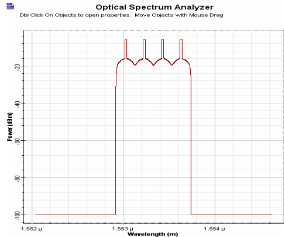
Fig. 8. The output of the proposed system with the smaller bandwidth.
