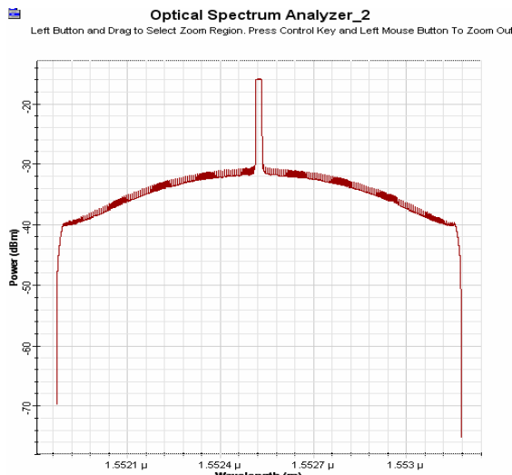
Fig. 6. The output of the 100 Gbps optical communication System
