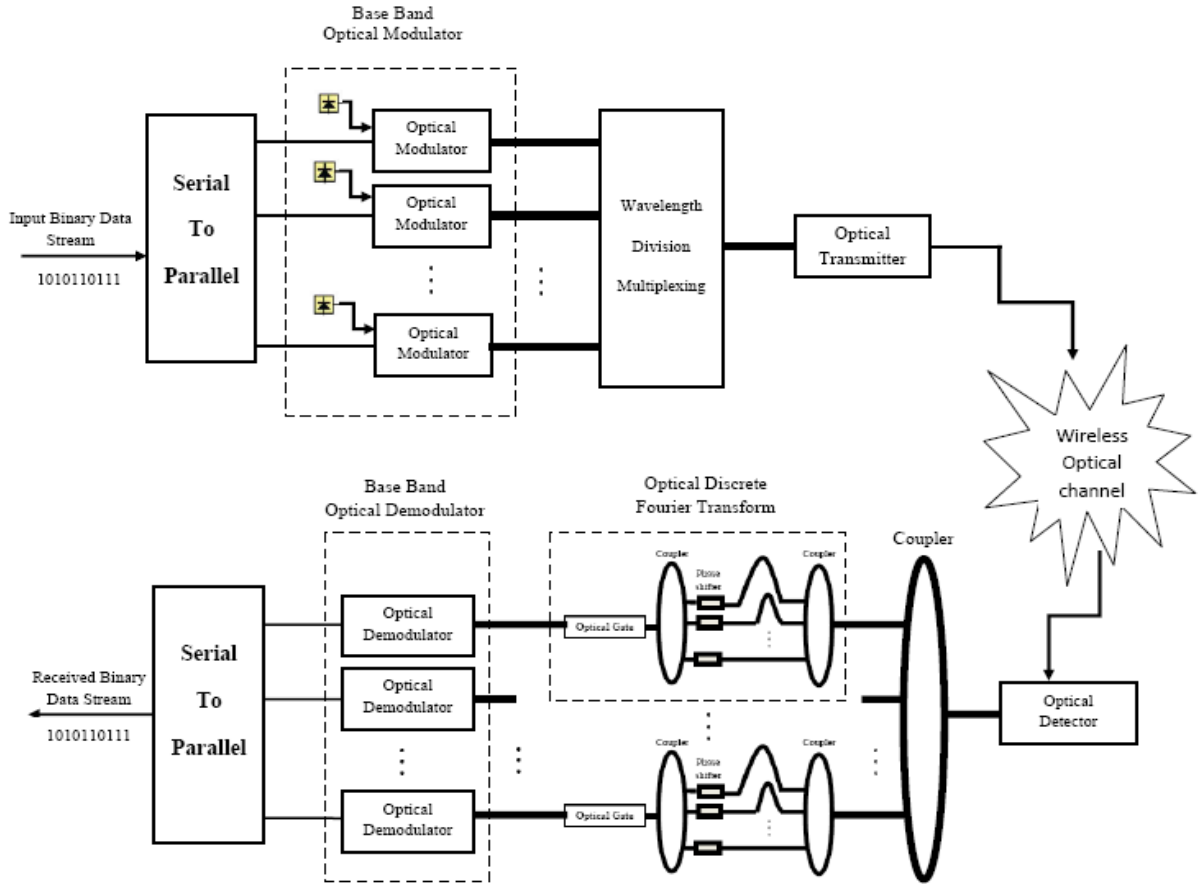
Fig. 2 Complete system architecture of all optical OFDM.
