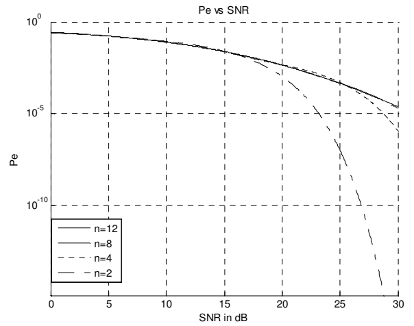
Fig. 4 Probability of error with signal to noise ratio.
