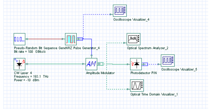
Fig. 5. 100 Gbps optical communication system.
