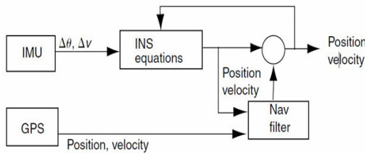
Figure 13 GPS/INS integration
