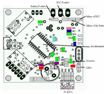
Figure 11 Main control board
