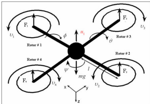
Figure 3 basic drawing of a Quadrotor showing the acting forces and moments
