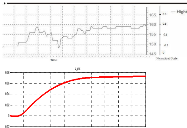
Figure 17 the comparison between the Simulink model and the hardware
