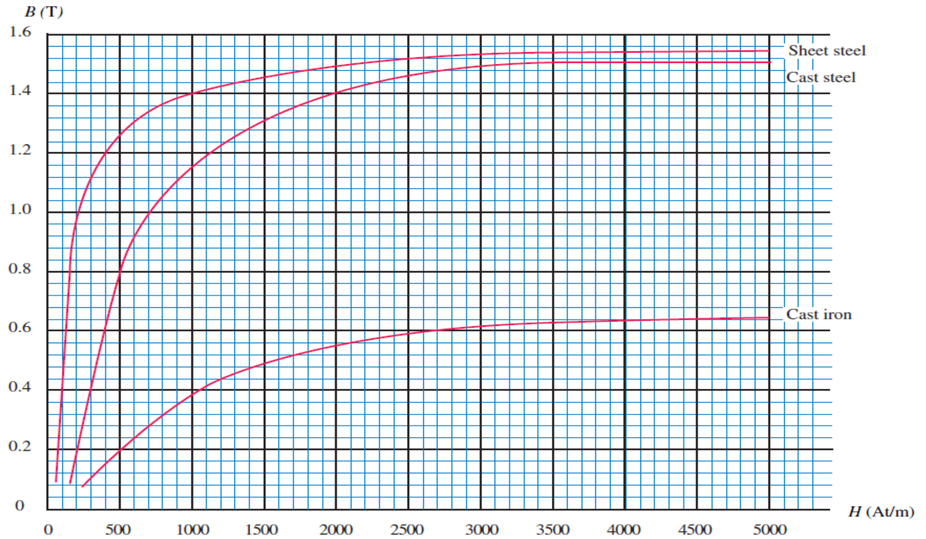
FIGURE 12-19 B - H curves for selected materials.
