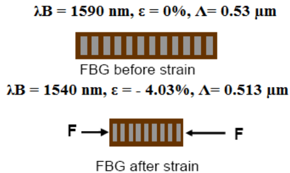
Fig. 6-a. Compression strain on FBG.
