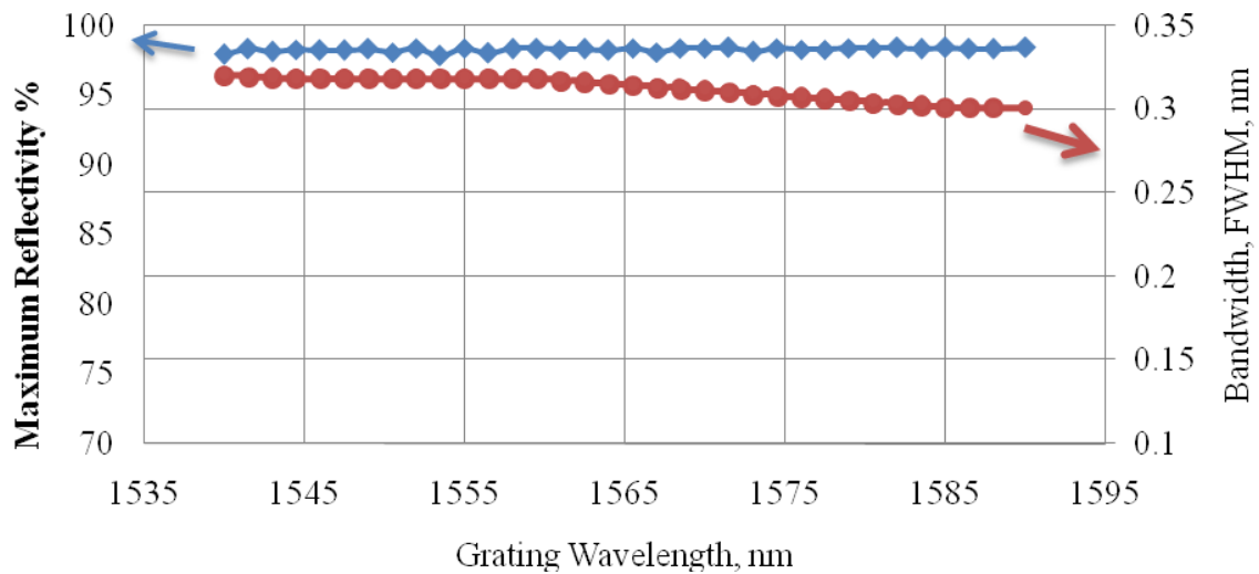
Fig.7. FBG peak reflectivity and (FWHM) bandwidth variation during compression.
