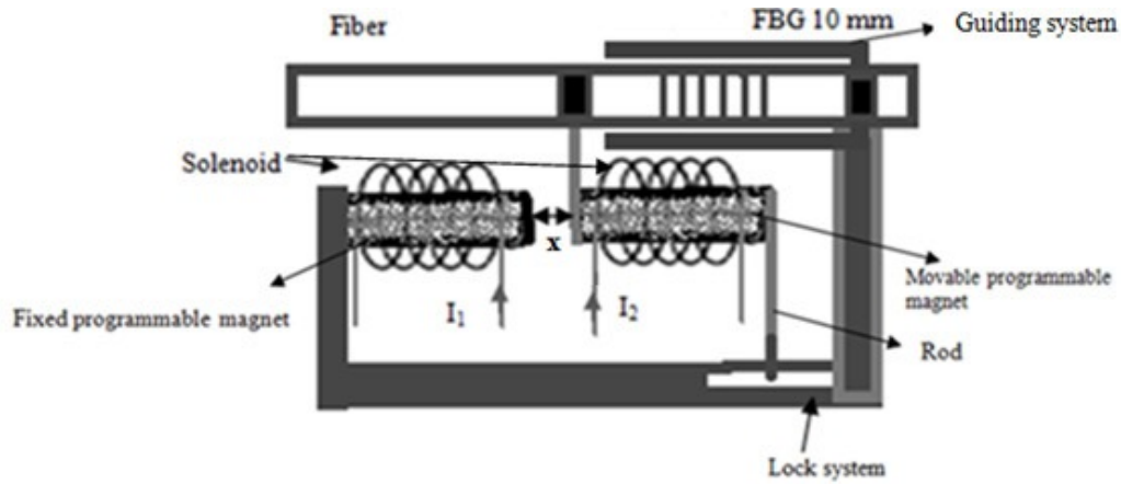
Fig. 1 Schematic of magnetically-tunable fiber Bragg grating device.
