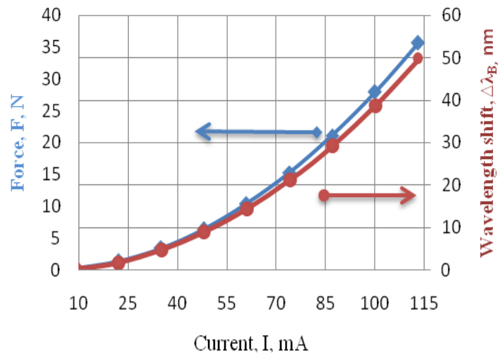
Fig. 2 The electromagnetic force and grating wavelength shift against solenoid current.
