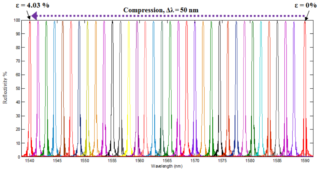
Fig. 6-b. Reflectivity of a 10 mm FBG during compression.
