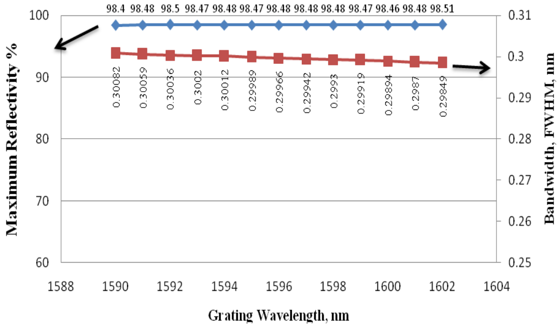
Fig. 5. FBG peak reflectivity and (FWHM) bandwidth variation during stretching.
