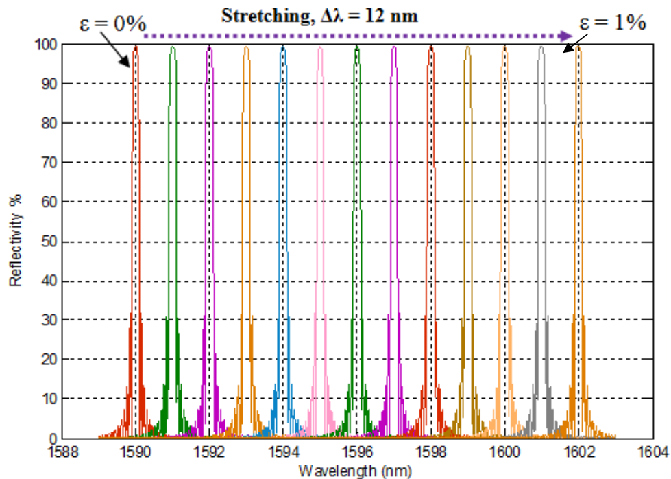
Fig. 4-b. Reflectivity of a 10 mm FBG during stretching.
