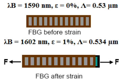
Fig. 4-a. Tension strain on FBG.
