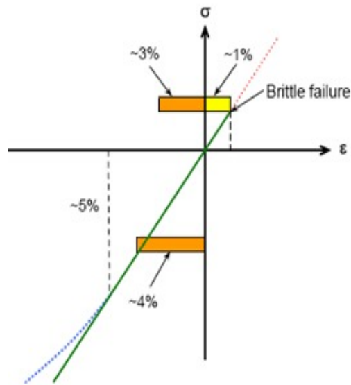
Fig. 3 Stress-strain relationship for an optical fiber [12].
