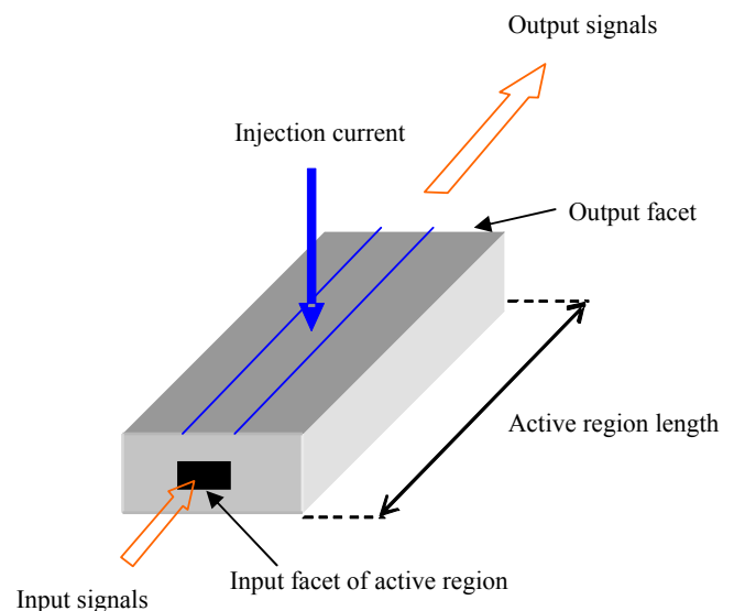
Fig. 1. Schematic diagram of the SOA.
