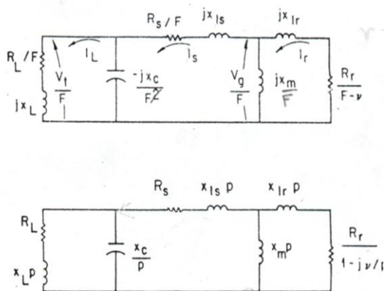
Fig. 2 Equivalent circuit of induction generator with load
