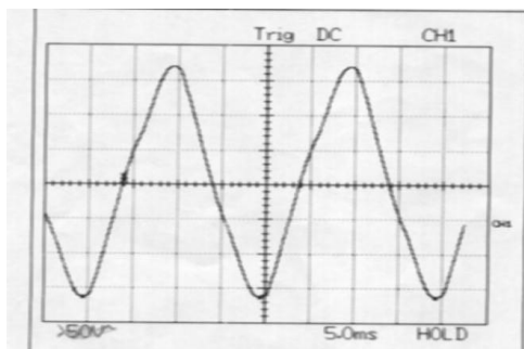
Fig.12 Experimental results of the load voltage
