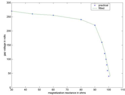
Fig. 3 Induction machine magnetization curve
