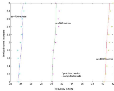
Fig. 6 Load current and frequency at different speeds
