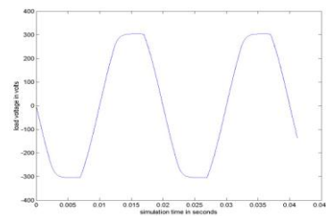
Fig. 9 Output line voltage of wind energy system
