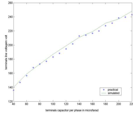
Fig. 4 The relationship between no load voltage and capacitor per phase at 1000 rev/min
