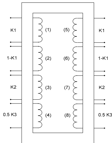
Fig. 12. Transformer Connection.
