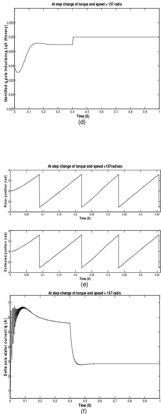
Figure 6. Position estimation and parameter identification error, under load change and speed = 157rad/s.
