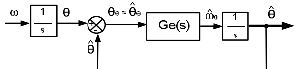
Figure 3. Equivalent block diagram of position and speed estimator.
