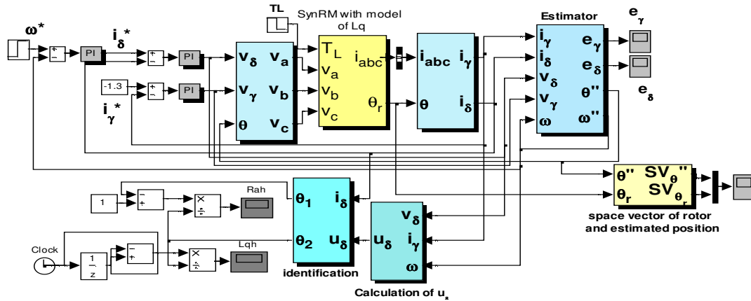
Figure 5. Simulink block diagram of SynRM vector control drive system with the proposed parameter identification scheme
