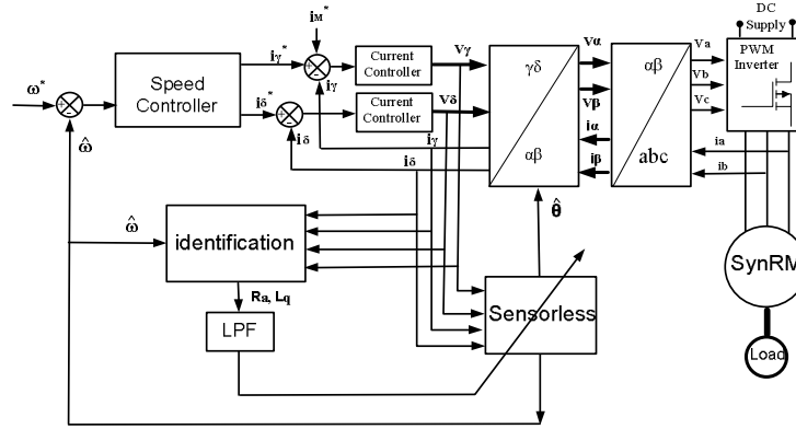
Figure 4. Block diagram of SynRM drive with the proposed on-line parameter identification system.
