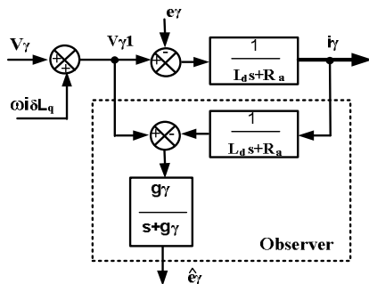
Figure 2. Equivalent block diagram of least-order observer for estimation of EEMF.
