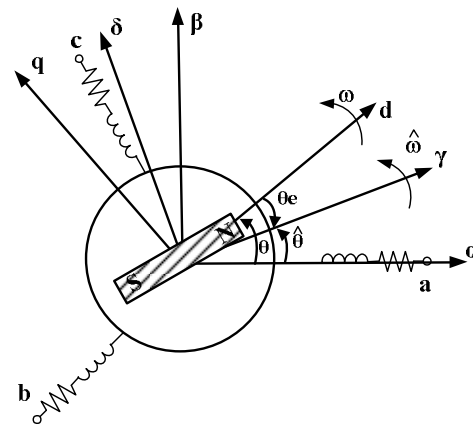
Figure 1. Coordinates of SynRMs.
