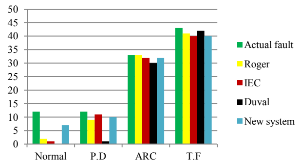
Figure 11. The three methods and new system statistics comparison.
