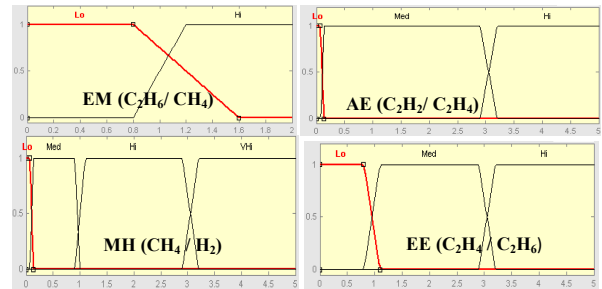
Figure 4. Roger’s fuzzy inputs membership function for gases ratio
