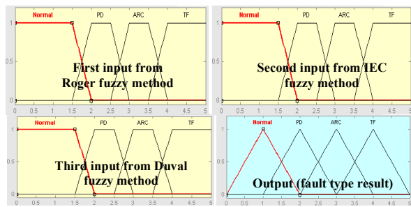
Figure 9. Grouping fuzzy controller three inputs and one output membership function.
