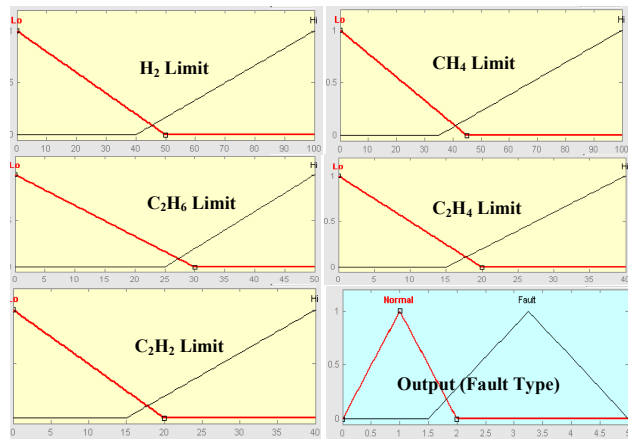
Figure 8. Normal limits fuzzy controller inputs and output membership; five gases ( H_2 , CH_4 , C_2H_6 , C_2H_4 and C_2H_2 ) and one output define its limits.
