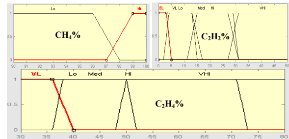
Figure 6. Duval fuzzy inputs with trapezoidal membership functions for gases ratio codes CH 4 %, C 2 H 2 % and C 2 H 4 %.
