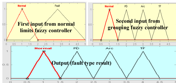
Figure 10. New fuzzy system controller two inputs and one output membership functions.
