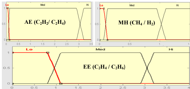
Figure 5. IEC fuzzy inputs membership function for gases ratio
