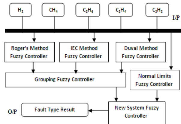
Figure 7. New fuzzy system technique block diagram.
