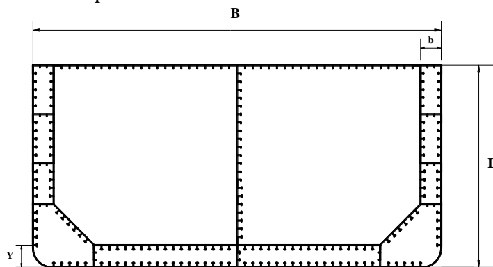
Figure 1: Actual mid-ship section of double hull oil tanker before damage.
