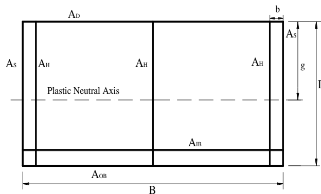
Figure 2: Idealized mid-ship of double hull oil tanker before damage.
