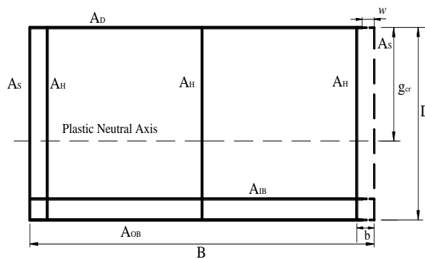
Figure 3: Structural configuration of double hull tanker after damage.
