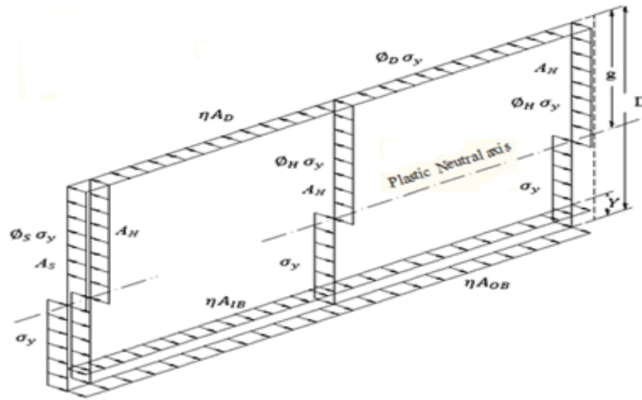
Figure 4: Equivalent average ultimate longitudinal stress distribution over the mid-ship section of an oil tanker in damaged condition.
